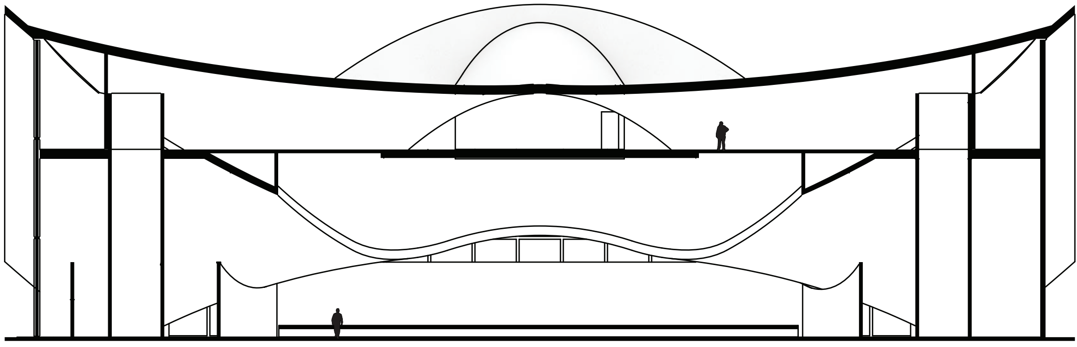
Section B 1:200
