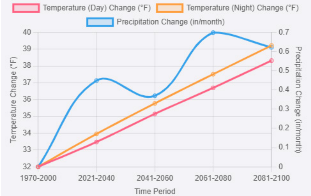
Climate Change Over Time (February) - SSP370 - ENSEMBLE MEAN
