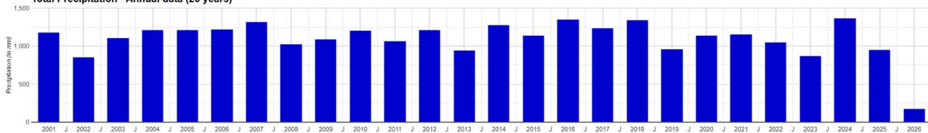
Total Precipitation - Annual data (25 years)
