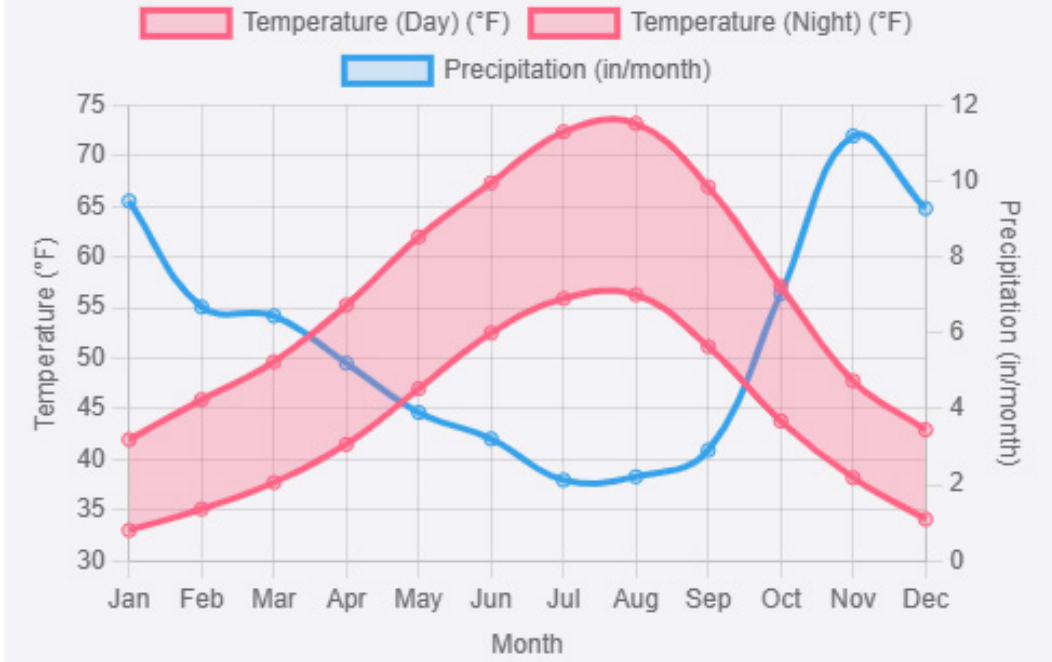
Climate by Month 1970-2000
